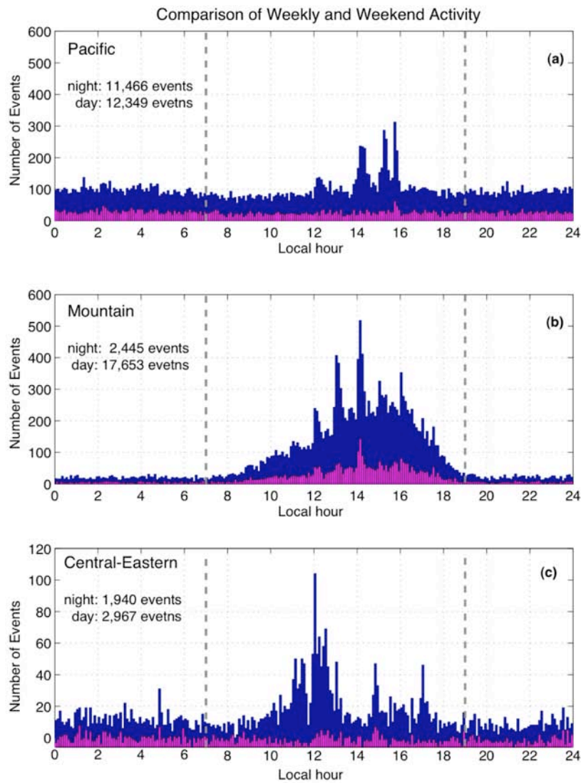
Figure 2: The blue bars show the result of stacking in 6-minute intervals all events occurred in a region as if they had occurred over a ‘virtual day’ in local time. The pink bars the resulting distribution if only events occurred on weekend days are considered. Each graph shows results for events occurred in different time zones: (a) Pacific, (b) Mountain, and (c) Central and Eastern. The number of events occurred in each region during local night and day hours are indicated. The vertical dash lines show our assumed local night/day boundary at 7 am, and the day/night boundary at 7 pm.
