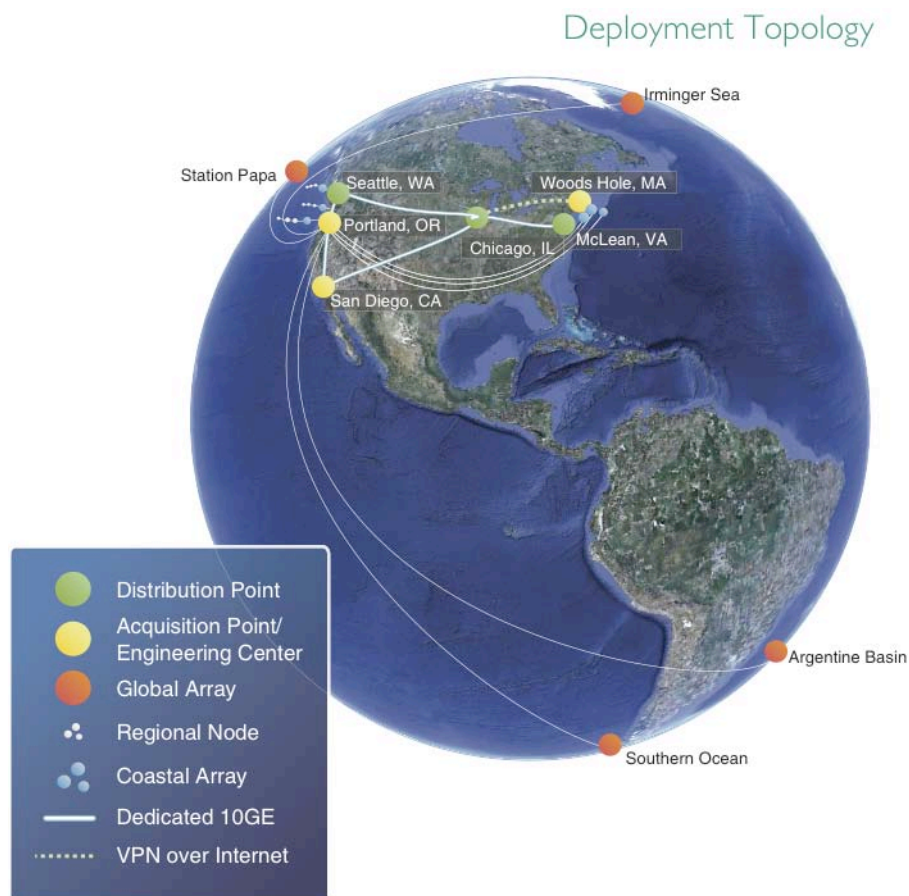
Figure 1: The OOI networks connecting platforms (e.g. buoys, autonomous vehicles, and seafloor cabled nodes) and sensors (e.g. seismometers, pH instruments and cameras) in the OOI. The primary continental network connects Seattle, Chicago, San Diego and Portland through a 10GE network in a triangular geometry which supports data transport from the primary acquisition point in Portland with the remainder of the network. The loss of a single connection or node in the network doesn't affect data flow. The design reliability of the network is 99.999%.
