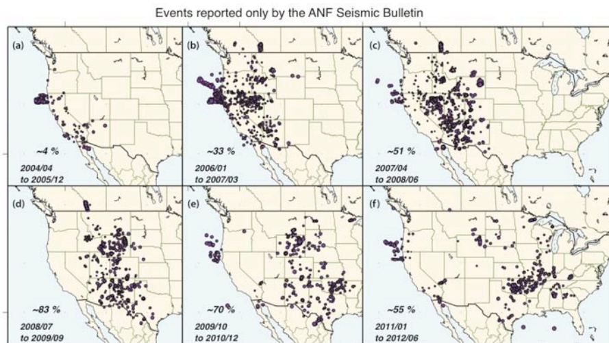
Figure 1: The map in each of the panels show the location of events reported only in the ANF Seismic Bulletin. The time period and the percentage of the unique events to the total number of events reported are indicated in the lower left side of each panel.
