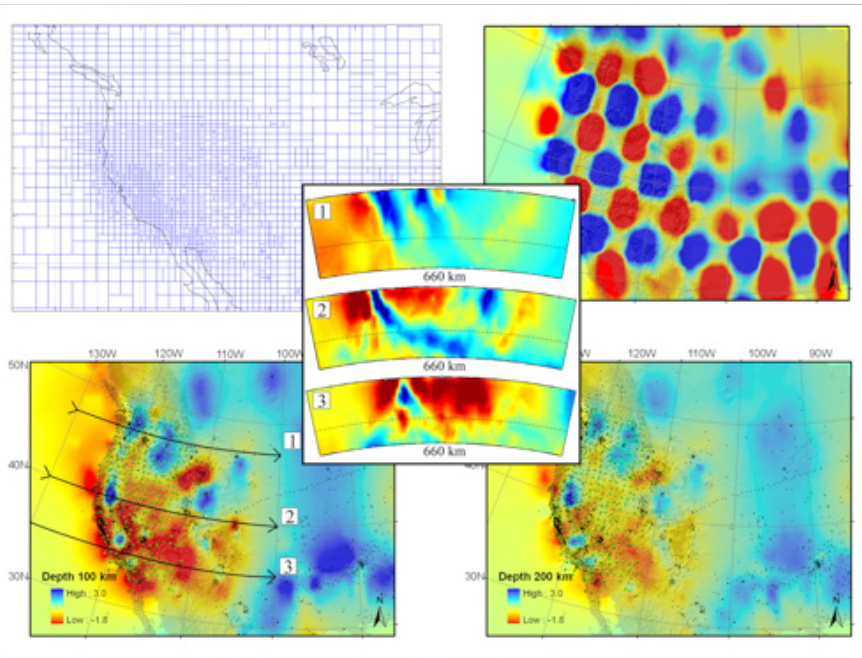
Figure 1. Results from body wave tomographic imaging using USArray. Top left the panels show grid resolution, top right checkerboard test, bottom shows map views at 100 km and 200 km depth. The middle panel shows three cross-sections.
