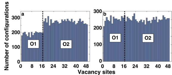
Figure 2: Oxygen vacancy distributions for the lower energy subsets of configurations of (a) Mg 16 Al 16 O 40 and (b) Ca 16 Al 16 O 40 perovskites (6 vacancies in 48 oxygen sites). Vacancies prefer to occupy the O2 sites in case a, and indicate no preference in case b.
