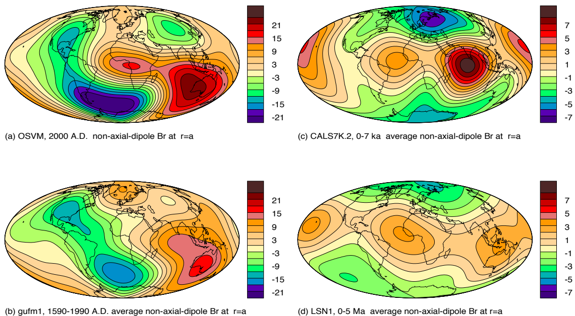
Figure 1: (a) Vertical component of the non-axial-dipole field in \mu T evaluated at Earth's surface using the geomagnetic field models OSVM for 2000A.D., (b) GUFM1 averaged over 400 years, (c) CALS7K.2 averaged over 7 kyr and (d) LSN1 averaged over 5 Myr. Note scales for (c) and (d) differ by factor of 3 from (a) and (b).
