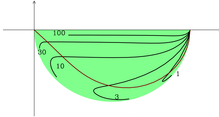
Figure 2: Contours of the smallest \|\sigma\|_2 \omega \mu_0 h^{3/2} in the complex c plane. Below the red line \sigma > 0 throughout; above it there is an insulating layer at the top.
