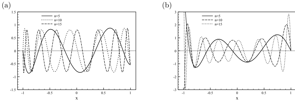
Figure 1: Plots of basis functions for n = 5, 10, 15 . In (a), \alpha = \beta = -1/2 and the functions satisfy the two-sided boundary conditions \Psi_n(-1) = \Psi_n(1) = 0 ; in (b), \alpha = \beta = 1/2 and the functions satisfy the one-sided boundary condition \Psi_n''(1) = \Psi_n(1) = 0 . Note the quasi-equal-area property of the functions in (b) and the quasi-equal-ripple property in (a).
