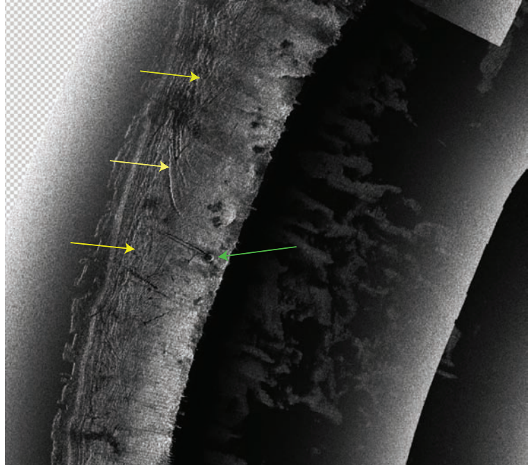
Side-scan sonar data from Fallen Leaf Lake (Tahoe basin), highlighting paleoshorelines (yellow arrows), and one of the many upright, submerged trees (green arrow) that casts a shadow (10 o'clock). This shadow is from a submerged pine tree with a bifurcated trunk that appears as two separate “drop outs” in the side-scan data! Many other trees and trunks are also visible in this image.
