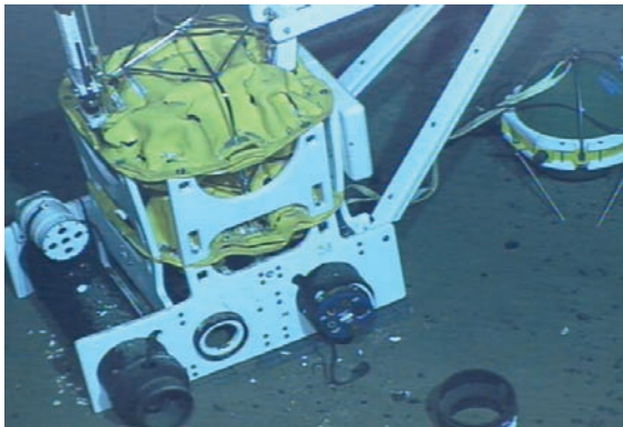
Figure 1: Catastrophic failure of broadband OBS at \approx 6\text{km} depth.
