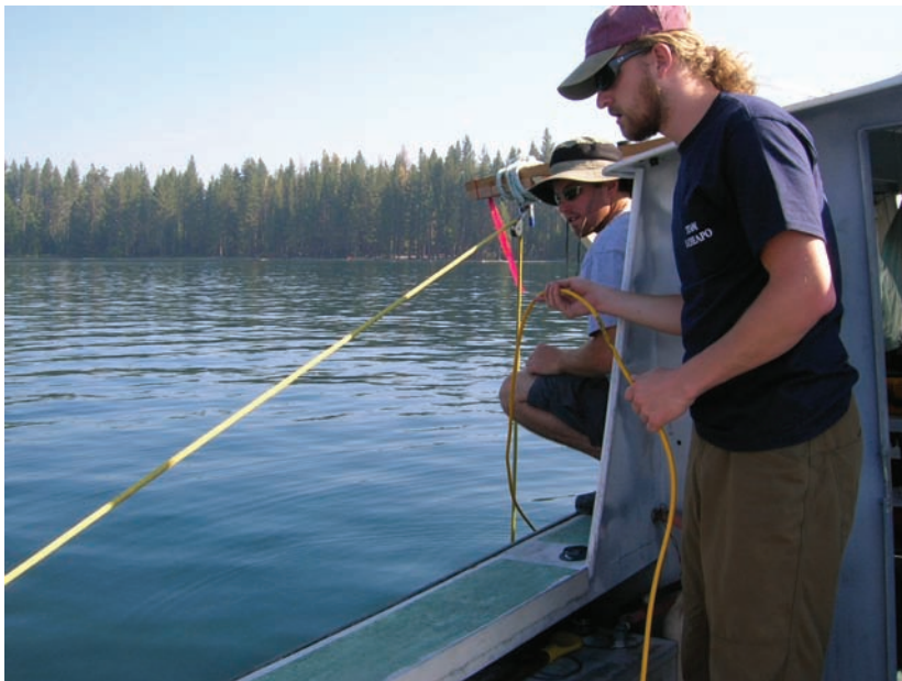
Graduate student Danny Brothers (left) and undergraduate summer intern Stefan Jensen (Northwestern University) deploy the side-scan sonar into the cobalt waters of Fallen Leaf Lake.
